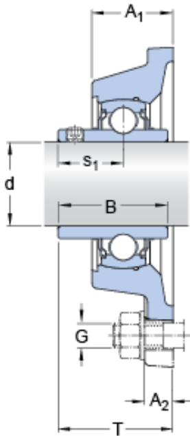
FY 35 TF/VA201 Bearing 2D drawings and 3D CAD models
